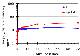
Figure 2: Mean plasma desmethyl-diazepam versus time in 12 subjects following a 10 mg dose rectally (filled red circles) and dermally by TDS diazepam (filled blue squares), logarithmic concentration axis.
